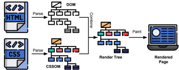
Figure 3: Rendering Path for Blink
