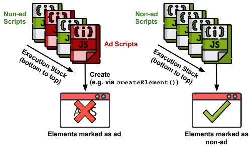
Figure 2: Execution projection for marking script-created ad elements
